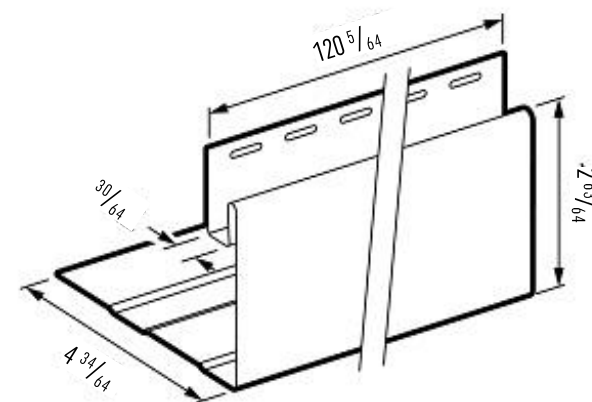
SV 17 Facade flashing small
