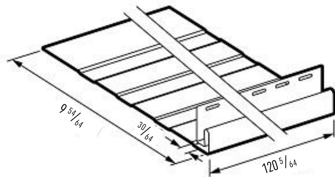
SV(P) 19 Facade flashing large
