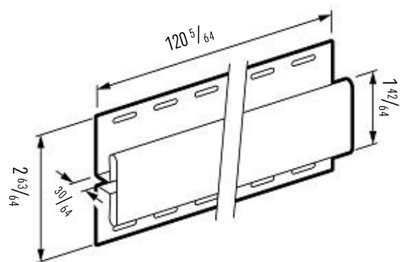
SV(P) 18 Connector
