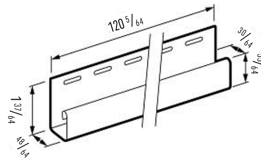
SV(P) 15 J-trim
