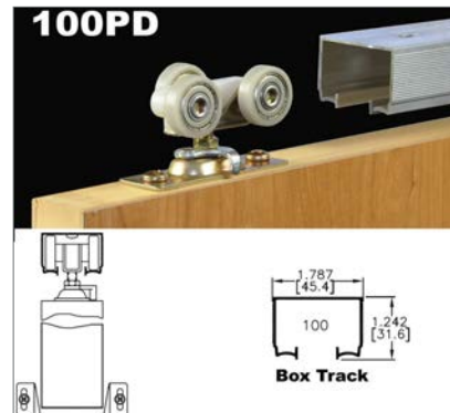
Pocket Door Hardware
