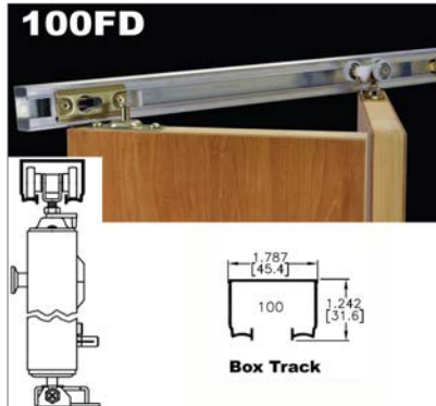
Bifold Door Hardware
