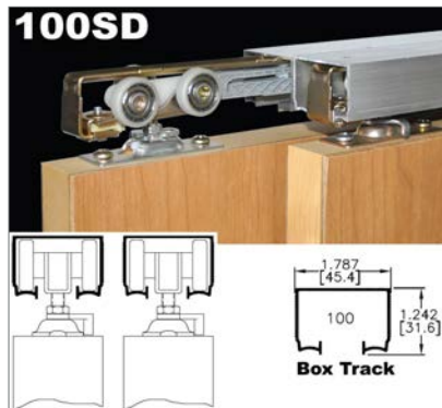
Sliding / Bypass Door Hardware
